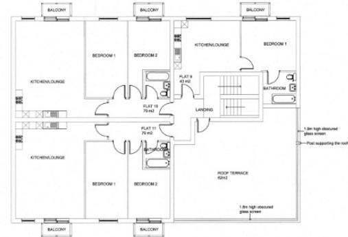
Proposed Second Floor Plan (Rear)
