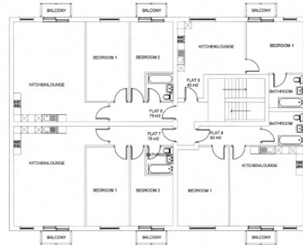
Proposed First Floor Plan (Rear)
