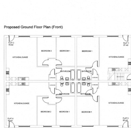
Proposed Ground Floor Plan (Front)
